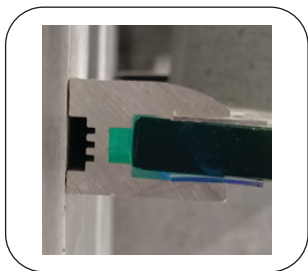
LEAL-511 Open LED Shelf Bracket For 12mm Glass (White/Blue) 300mm,450mm,600mm
